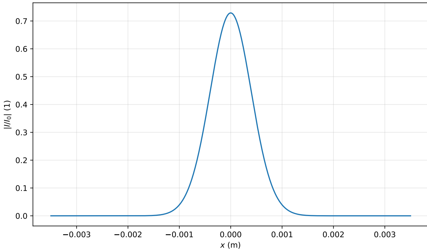
Intensity profile I(x, y = 0, z = 1.353m)/I_0 , P_{in}=0.1P_{cr} , artificial time
